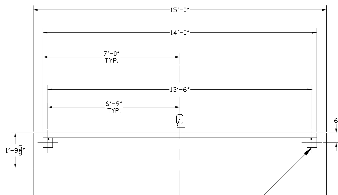
SECTION A-A END WALL/BUMPS
